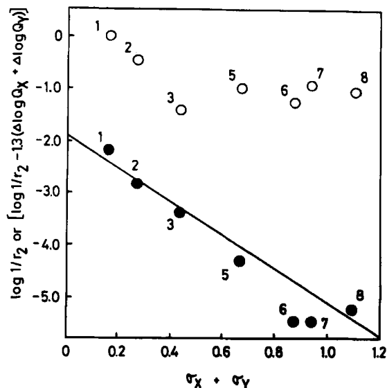
FIG. 3. Effects of \alpha -substituents on the reactivities of the crotonyl monomers toward poly-AN radical: (○) plot of \log(1/r_2) vs. (\sigma_X + \sigma_Y) ; (●) plot of [\log(1/r_2) - 1.3(\Delta\log Q_X + \Delta\log Q_Y)] vs. (\sigma_X + \sigma_Y) . Numbers are same as in Table 1.
