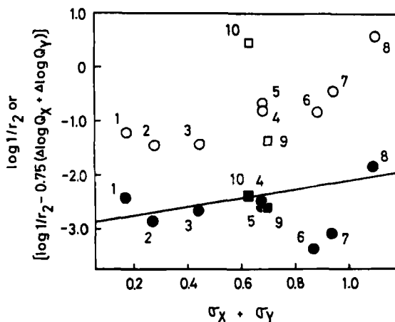
FIG. 2. Effects of \alpha -substituent on the reactivities of the crotonyl monomers toward poly-St radical: (○) and (◻) plot of \log (1/r_2) vs. (\sigma_X + \sigma_Y) ; (●) and (◼) plot of [\log (1/r_2) - 0.75(\Delta \log Q_X + \Delta \log Q_Y)] vs. (\sigma_X + \sigma_Y) . Numbers are same as in Table 1.
